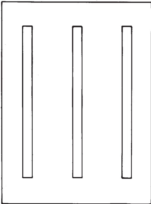
Figure 13.16 Linear pattern, continuous 1 ft × 4 ft rectilinear luminaires.
