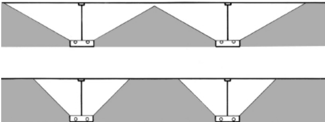
Figure 13.21 Above, properly located indirect luminaires with wide distributions produce even luminance; below, improperly located indirect luminaires with narrow distributions produce areas of uneven luminance.
