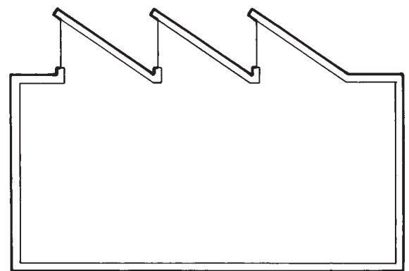
Figure 5.9 Sawtooth section.
