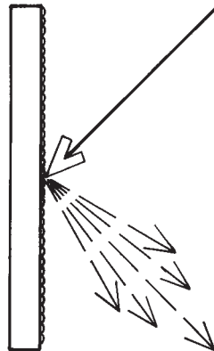
Figure 9.2 Semi-specular (spread) reflection.
