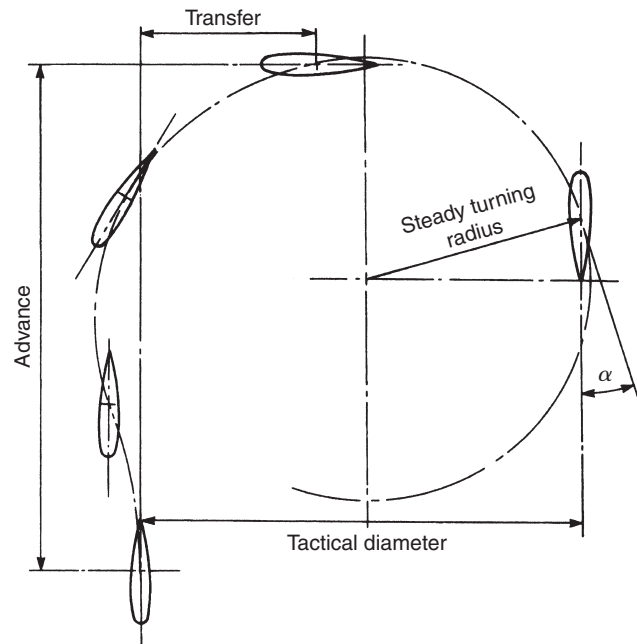
Figure 13.1 Turning circle
