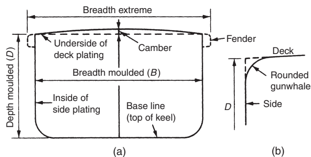
Figure 3.2 Breadth measurements
