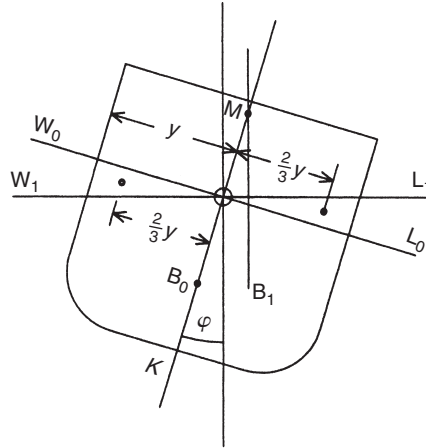
Figure 5.7 Transverse metacentre
