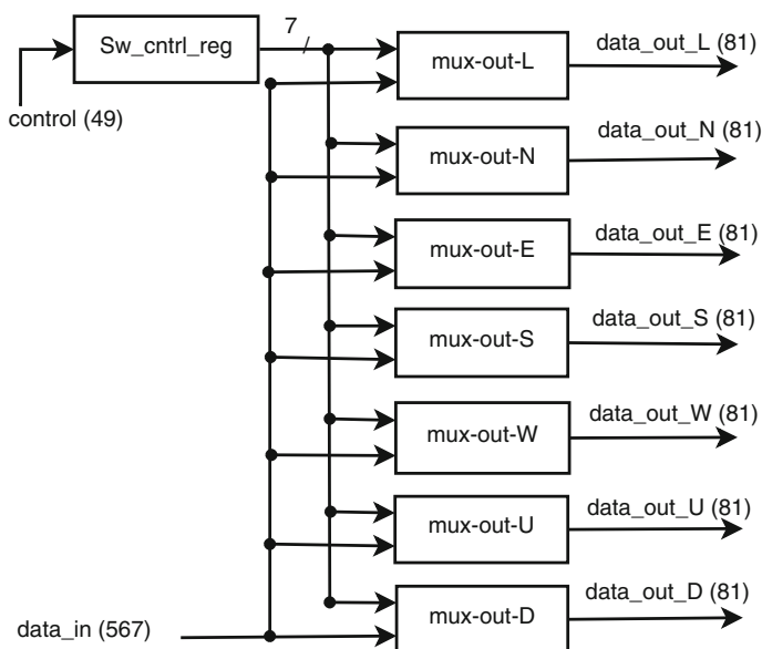
Fig. 5.10 Crossbar circuit
