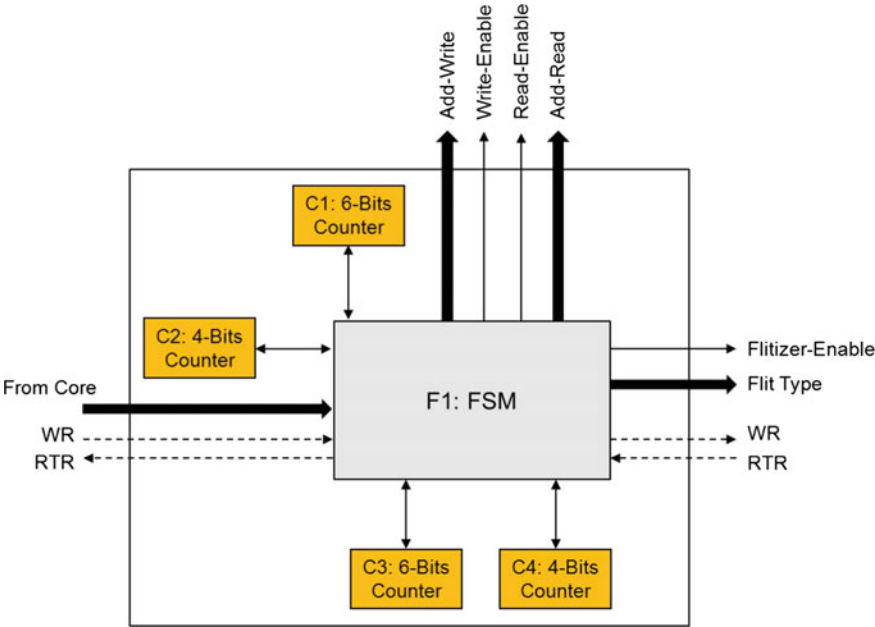
Fig. 4.43 Core-to-router (C2R) controller architecture
