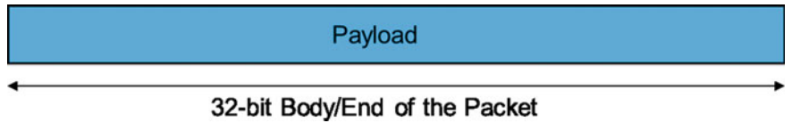
Fig. 4.39 Format of BODY/END flits after deflitzization
